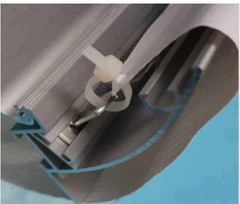
Fixing flex banner with slide fastener
