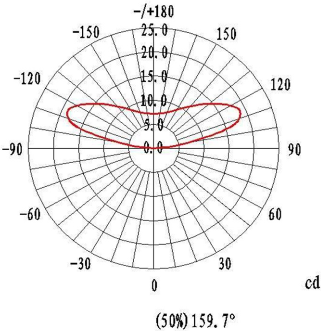
LIGHT DISTRIBUTION
