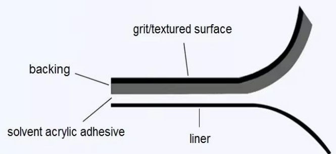
Structure Image of Anti Slip Tape
