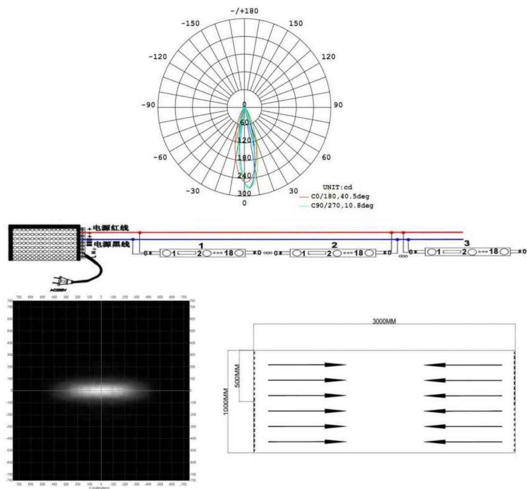
LUMINOUS INTENSITY DISTRIBUTION DIAGRAM
